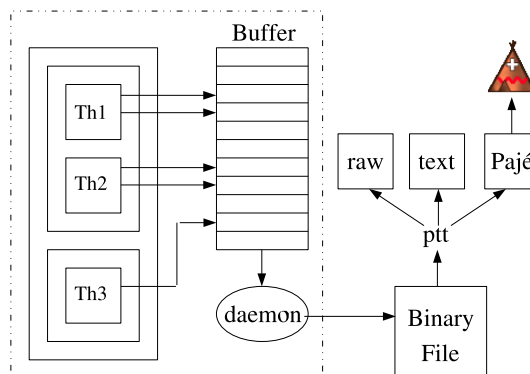
Figure 3: Architecture
