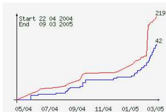
Figure 2: Project progression
