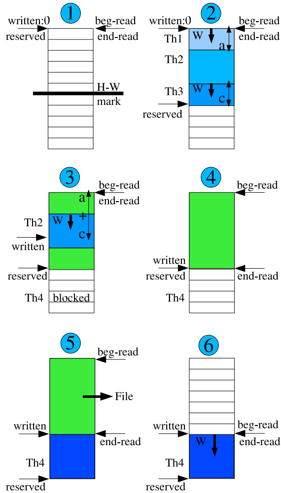
Figure 4: Buffer management
